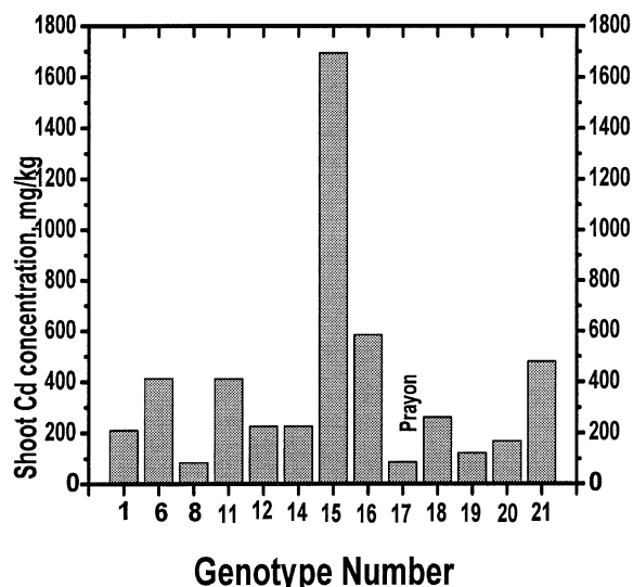
Fig. 3. Variation in Cd in shoots of Thlaspi caerulescens ecotypes from different locations in Europe when grown on soil at Palmerton, PA which contained 158 mg Cd and 15,500 mg Zn/kg dry soil and pH 6.0 in water (Chaney et al. 2000); genotypes 15, 16, 21, 6 and 8 were from southern France, while genotype 17 was from Prayon, Belgium, and genotypes 8, 19 and 20 were from the UK.
